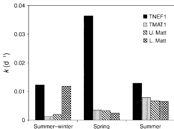
FIG. 7. Mean leaf decomposition rates ( k ) from a forested watershed (TNEF1), from a reclaimed mine (TMAT1), from the confluence of TMAT1 and Matthews Run (L. Matt), and from Matthews Run above the confluence (U. Matt). The summer-winter incubation period was July 2001 through March 2002 (228 days), the spring period was March through July 2002 (129 days), and the summer period was July through October 2002 (96 days).
