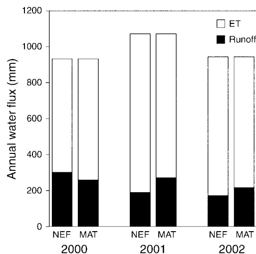
FIG. 3. Annual water flux (evapotranspiration [ET] and runoff) from NEF and MAT watersheds for water years ending in 2000–2002. The height of each bar represents annual precipitation.
