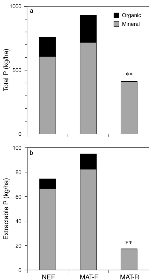
FIG. 2. (a) Total soil P pools and (b) bicarbonate-extractable (plant-available) P pools in a forested watershed (NEF), the forested portion of a mined watershed (MAT-F), and the mined and reclaimed portion of a mined watershed (MAT-R). Pools were measured 15 years after reclamation was completed to a depth of 10 cm.
