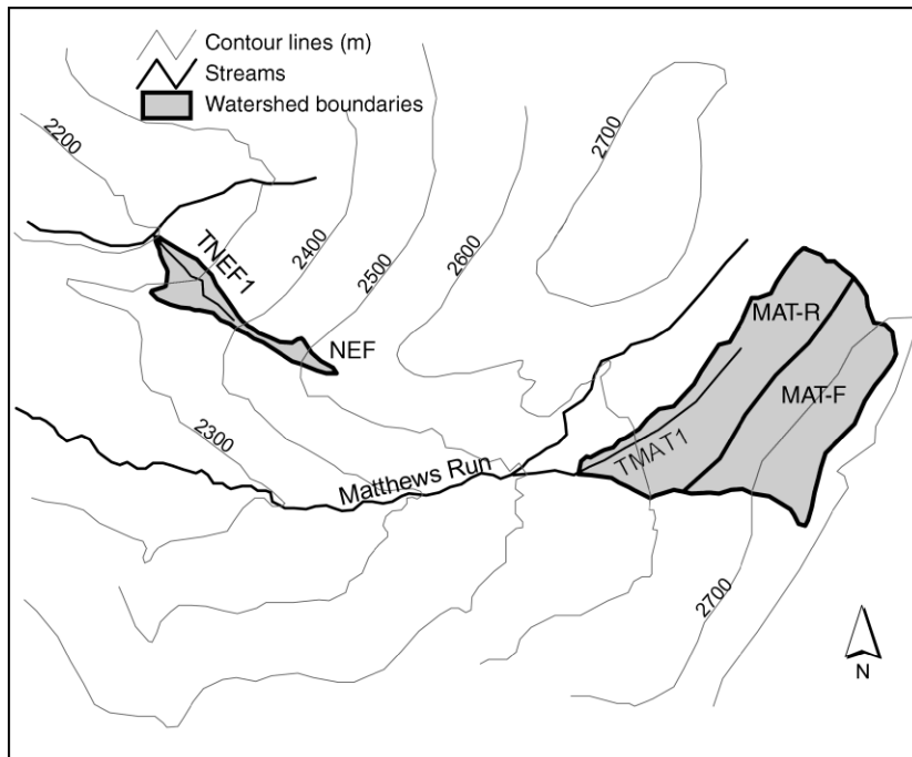
FIG. 1. Topographic map showing the relative locations of the watersheds of the study area in western Maryland, USA. TNEF1 is the stream that drains NEF watershed. TMAT1 is the stream that drains MAT watershed. TMAT1 is a tributary of Matthews Run. MAT is subdivided into a reclaimed mine section (MAT-R) and a forested section (MAT-F).
