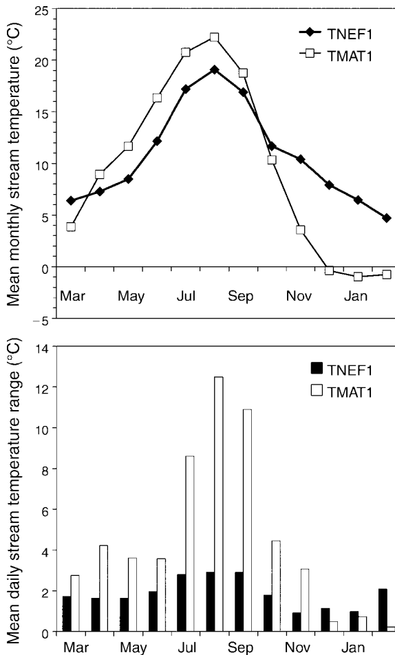
FIG. 6. Mean monthly stream temperature and mean daily range of stream temperature for TNEF1 and TMAT1 from March 2001 to February 2002.
