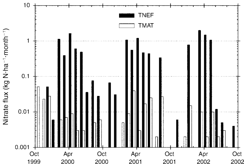
FIG. 5. Monthly runoff flux of nitrate from TNEF1 and TMAT1 from October 1999 through September 2002. Note the y-axis log scale.
